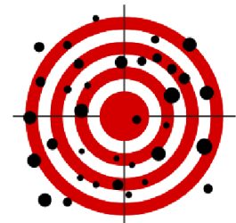
Unreliable, But Valid
