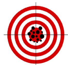
Both Reliable & Valid
